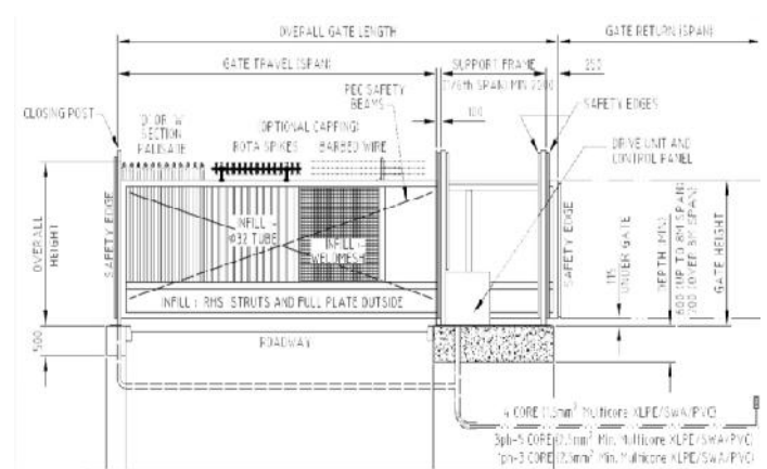
BS EN12453 – Areas of risk on gates
