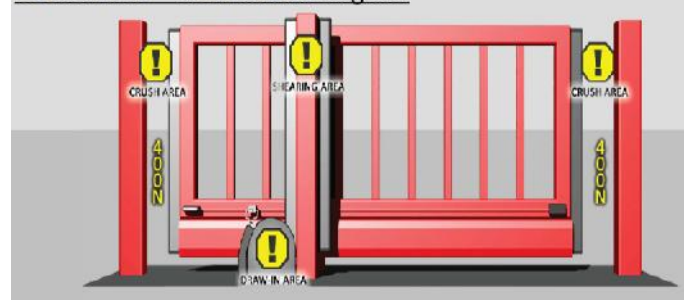
BS EN12453 – Areas of risk on gates
